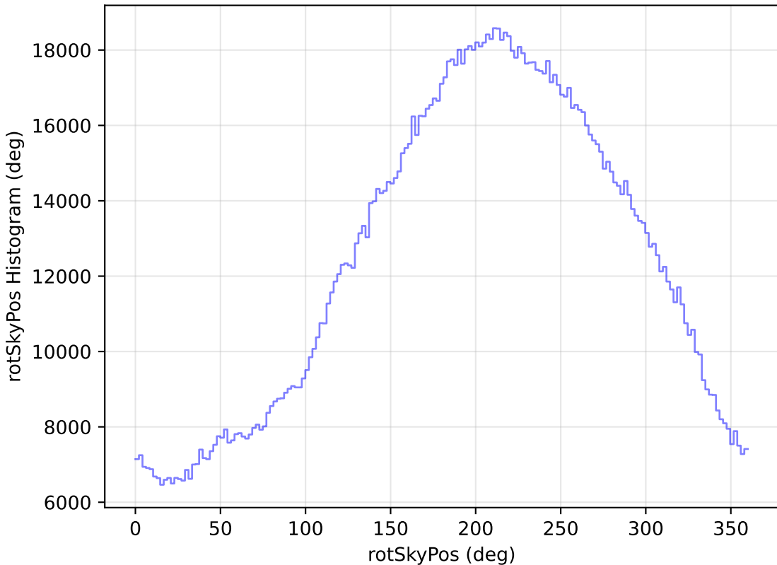
too_elab_r8_d2_ugrizy_v3.4_10yrs All sky all bands: rotSkyPos Histogram
