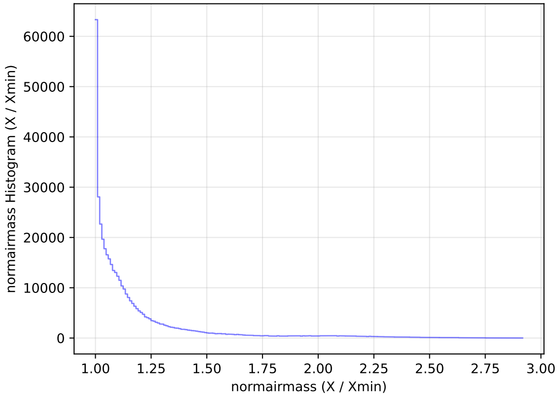
too_elab_r8_d2_ugrizy_v3.4_10yrs WFD z band: normairmass Histogram
