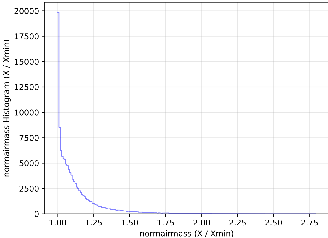
too_elab_r8_d2_ugrizy_v3.4_10yrs WFD u band: normairmass Histogram
