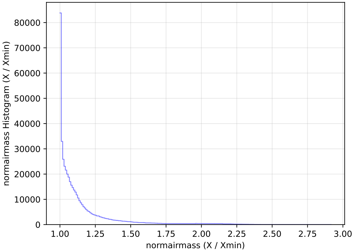
too_elab_r8_d2_ugrizy_v3.4_10yrs WFD r band: normairmass Histogram
