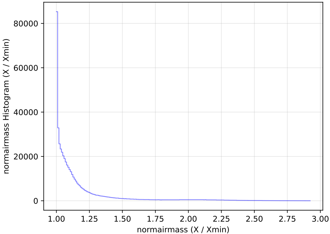
too_elab_r8_d2_ugrizy_v3.4_10yrs WFD i band: normairmass Histogram
