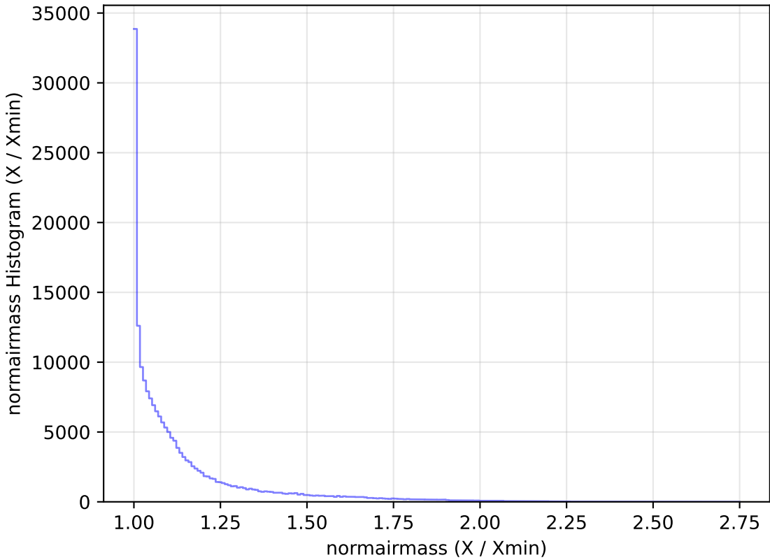
too_elab_r8_d2_ugrizy_v3.4_10yrs WFD g band: normairmass Histogram
