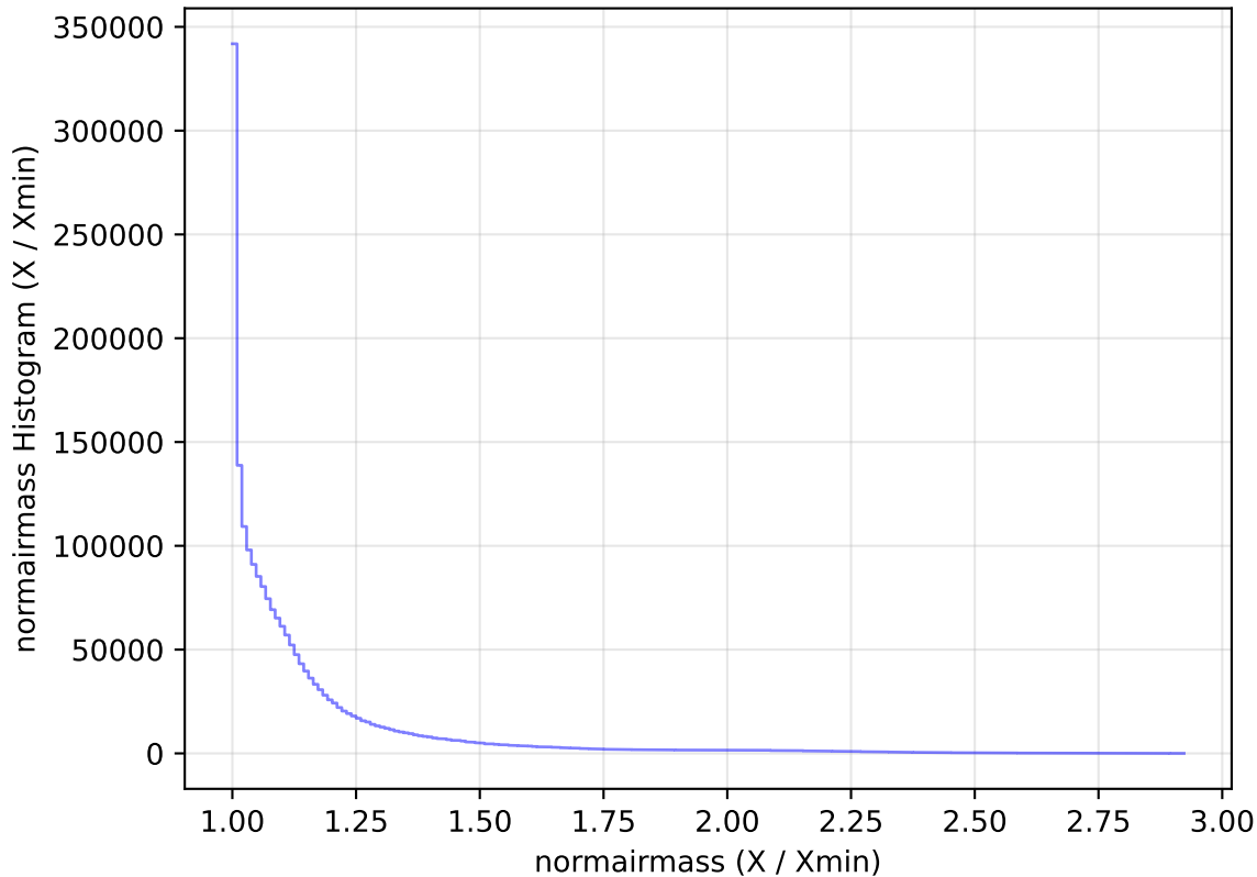
too_elab_r8_d2_ugrizy_v3.4_10yrs WFD all bands: normairmass Histogram
