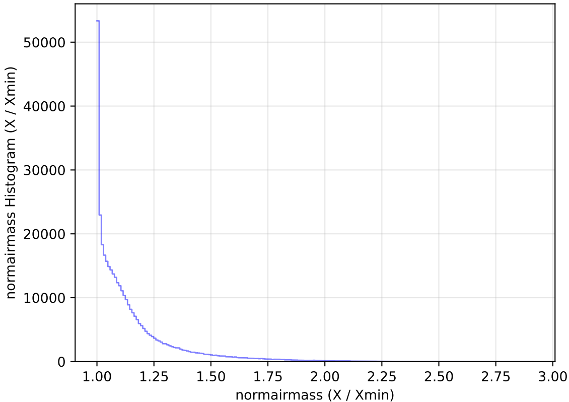
too_elab_r8_d2_ugrizy_v3.4_10yrs All sky y band: normairmass Histogram
