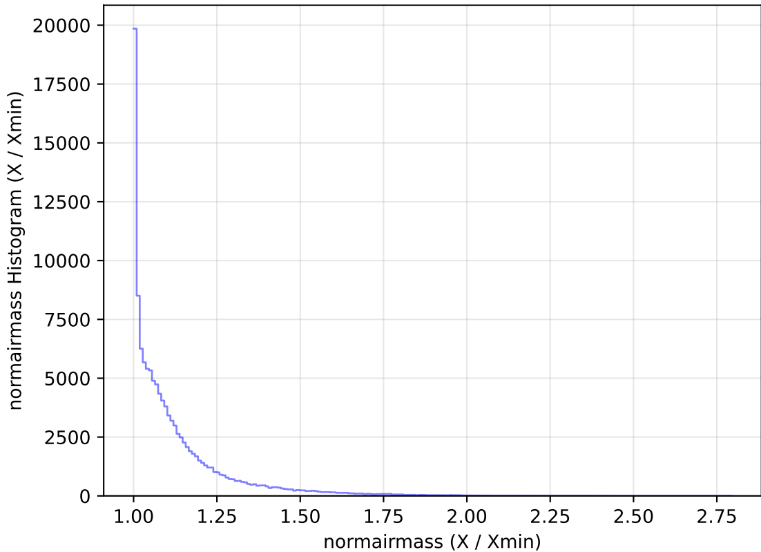
too_elab_r8_d2_ugrizy_v3.4_10yrs All sky u band: normairmass Histogram
