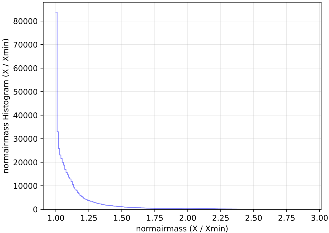
too_elab_r8_d2_ugrizy_v3.4_10yrs All sky r band: normairmass Histogram
