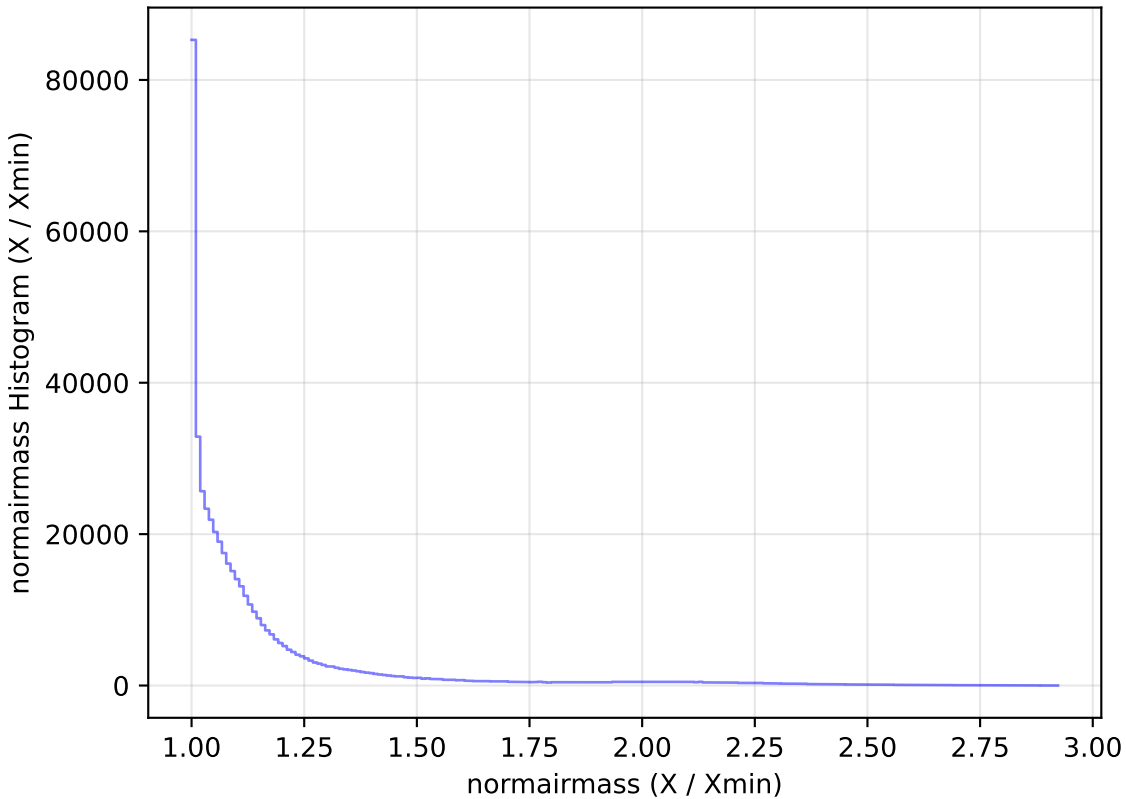
too_elab_r8_d2_ugrizy_v3.4_10yrs All sky i band: normairmass Histogram
