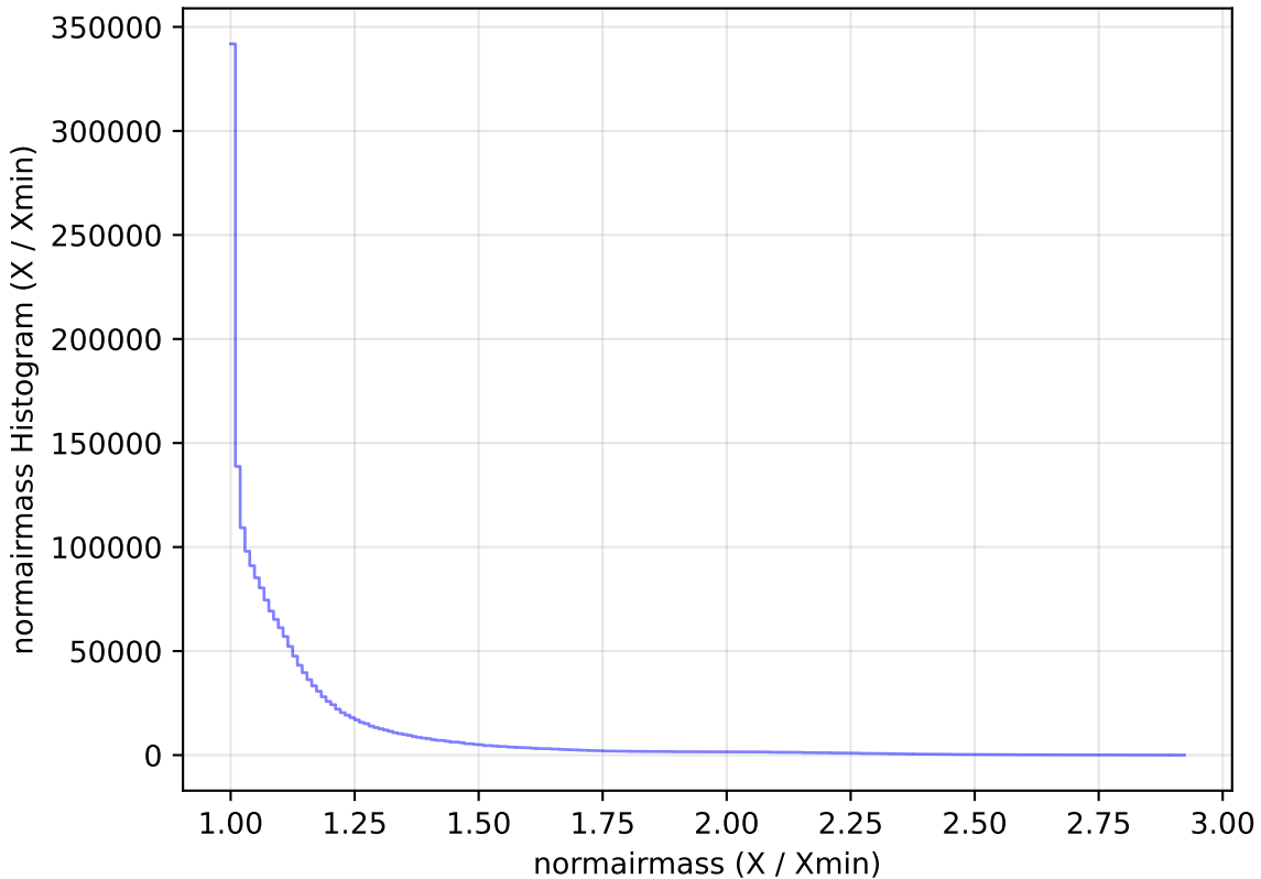
too_elab_r8_d2_ugrizy_v3.4_10yrs All sky all bands: normairmass Histogram
