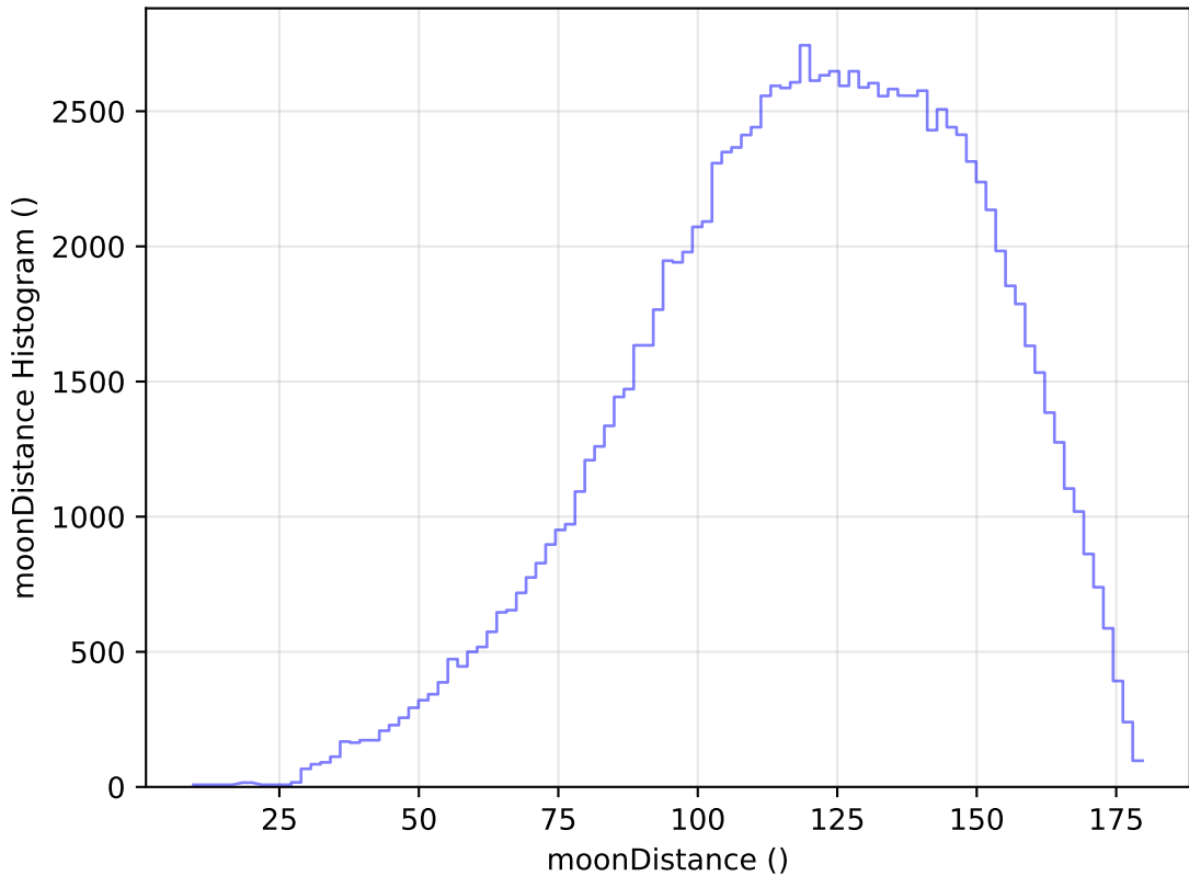
too_elab_r8_d2_ugrizy_v3.4_10yrs WFD u band: moonDistance Histogram
