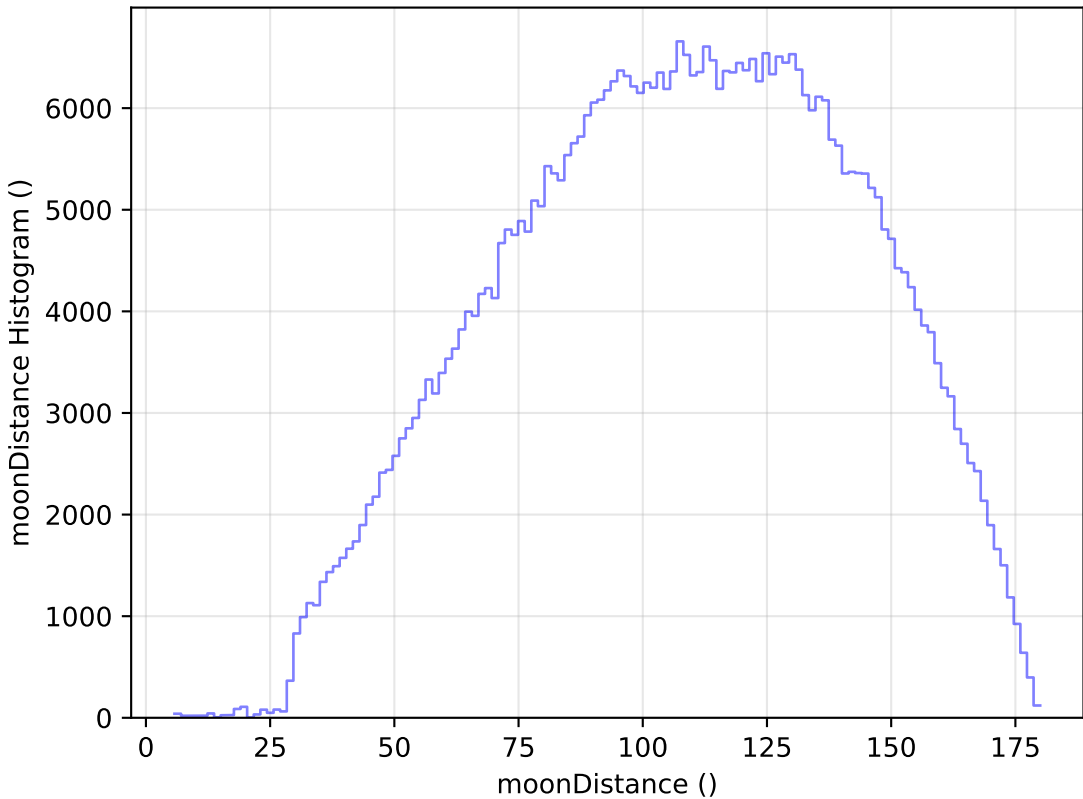
too_elab_r8_d2_ugrizy_v3.4_10yrs WFD r band: moonDistance Histogram
