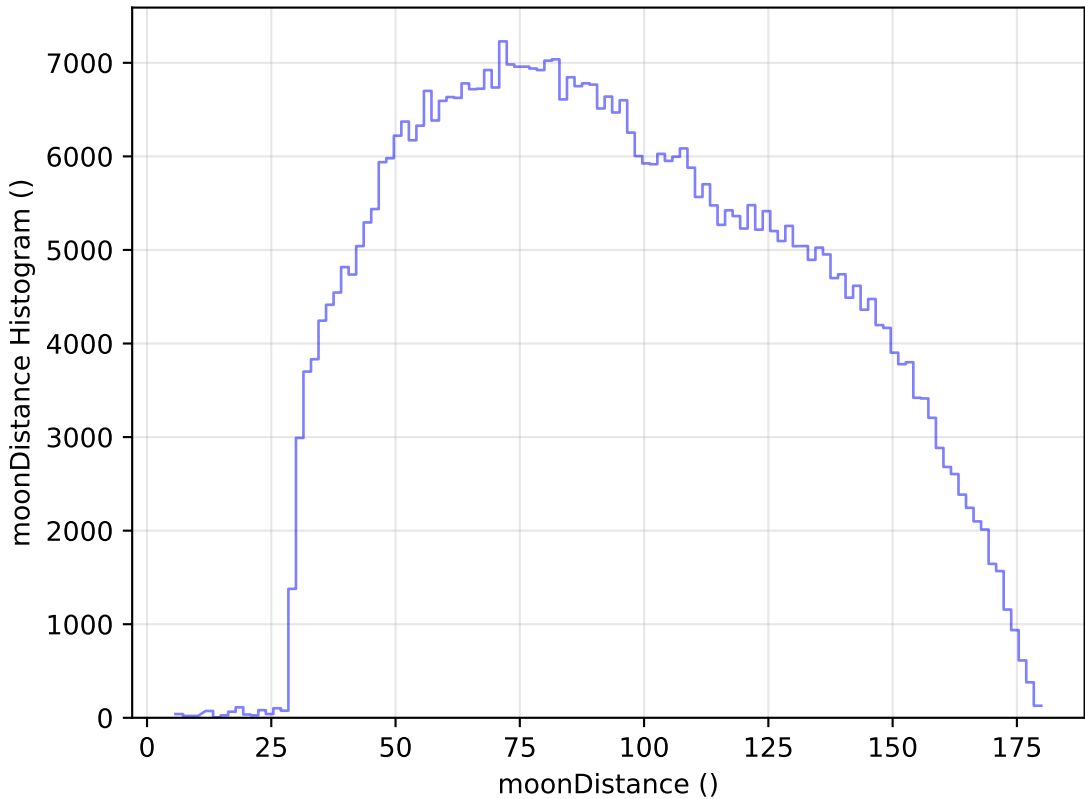
too_elab_r8_d2_ugrizy_v3.4_10yrs WFD i band: moonDistance Histogram
