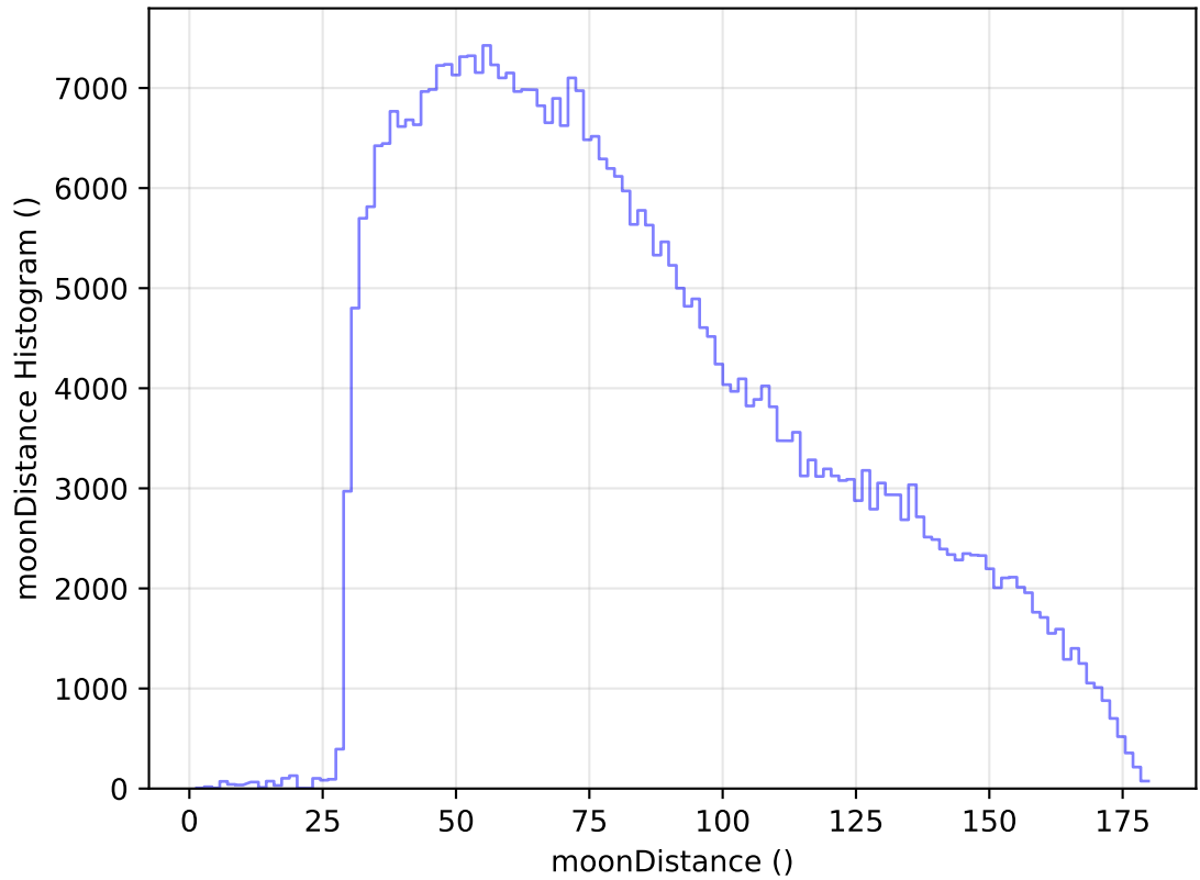
too_elab_r8_d2_ugrizy_v3.4_10yrs All sky z band: moonDistance Histogram
