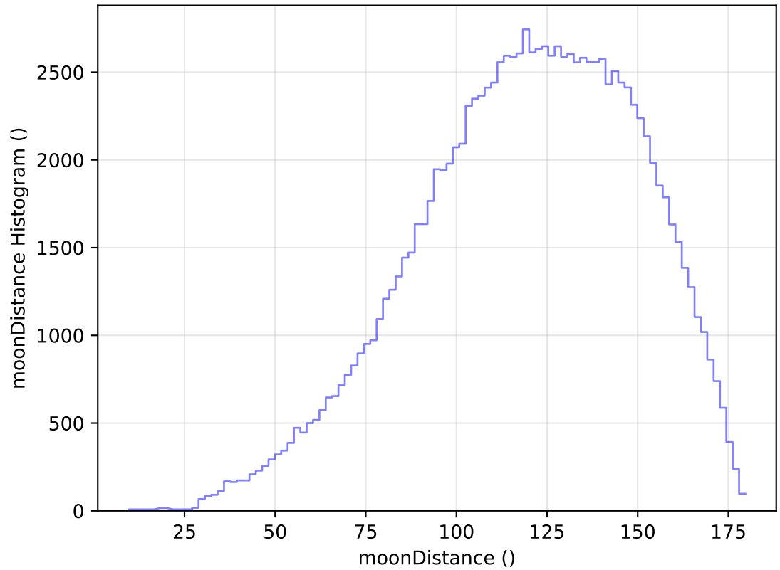
too_elab_r8_d2_ugrizy_v3.4_10yrs All sky u band: moonDistance Histogram
