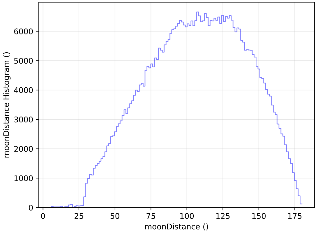
too_elab_r8_d2_ugrizy_v3.4_10yrs All sky r band: moonDistance Histogram
