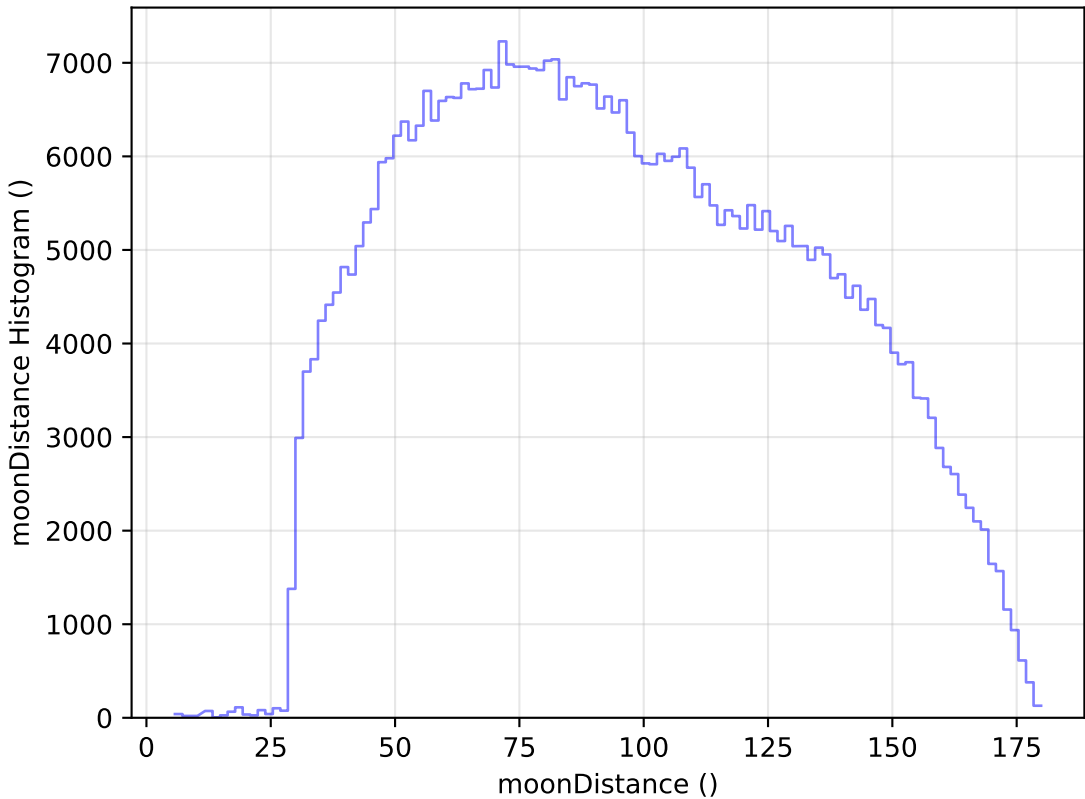
too_elab_r8_d2_ugrizy_v3.4_10yrs All sky i band: moonDistance Histogram
