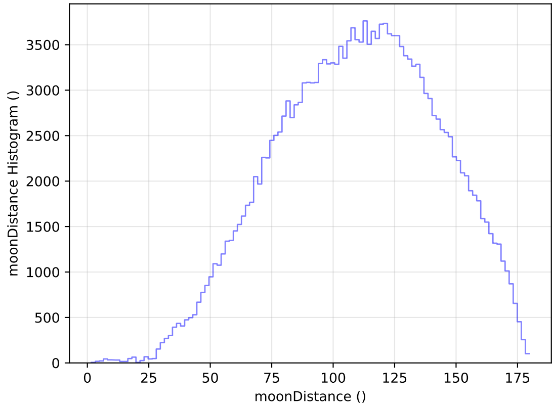
too_elab_r8_d2_ugrizy_v3.4_10yrs All sky g band: moonDistance Histogram
