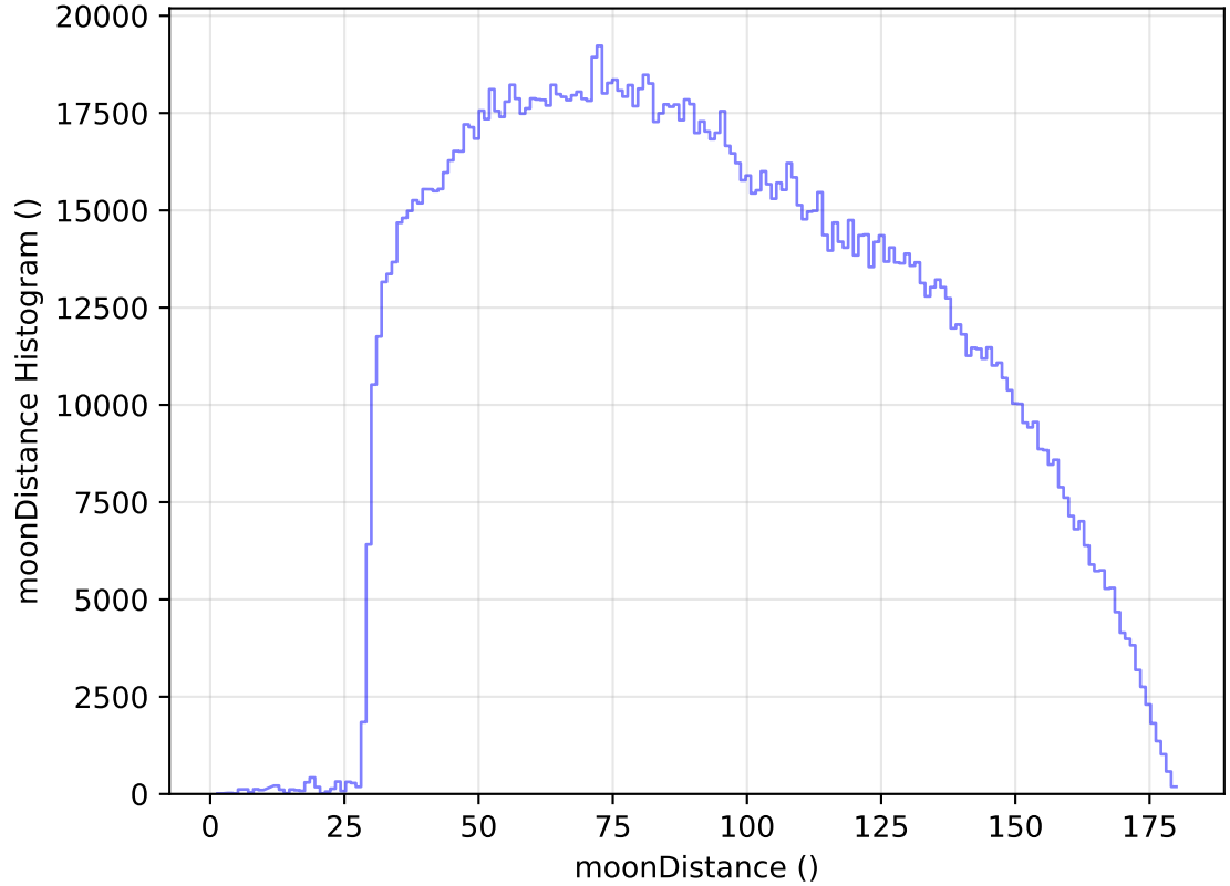
too_elab_r8_d2_ugrizy_v3.4_10yrs All sky all bands: moonDistance Histogram
