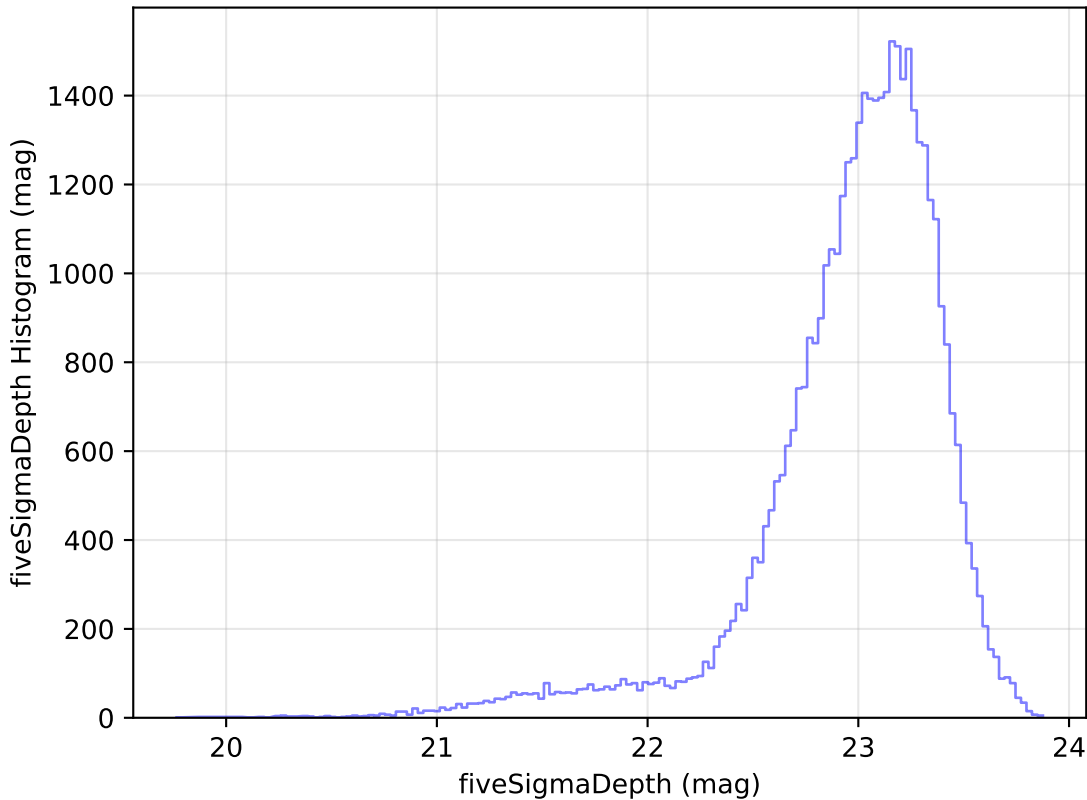
too_elab_r8_d2_ugrizy_v3.4_10yrs Yr 1 z band: fiveSigmaDepth Histogram
