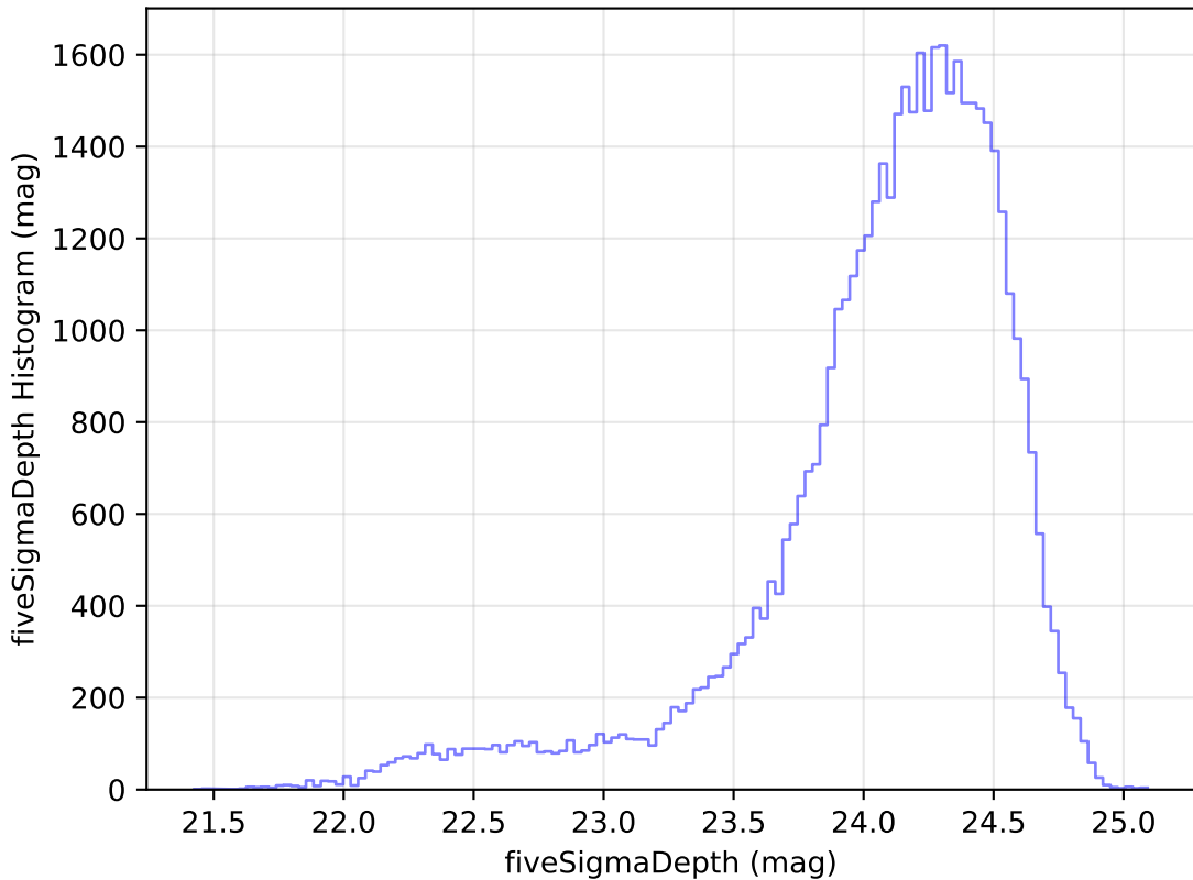
too_elab_r8_d2_ugrizy_v3.4_10yrs Yr 1 r band: fiveSigmaDepth Histogram
