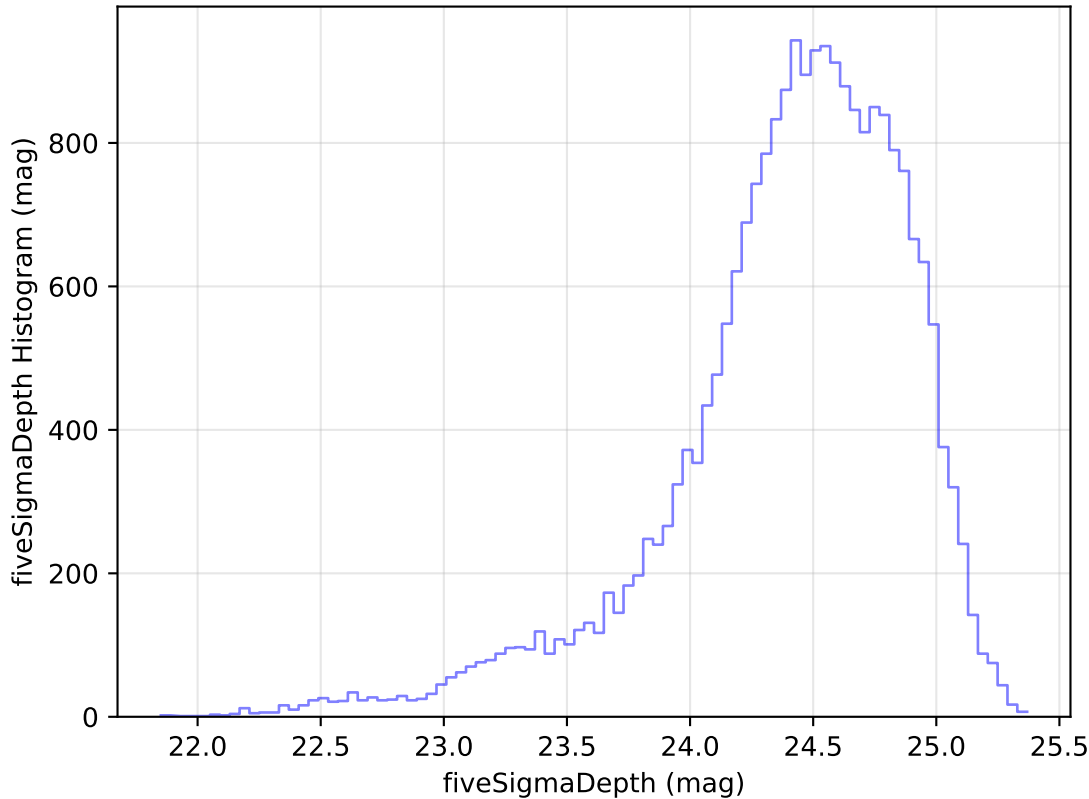
too_elab_r8_d2_ugrizy_v3.4_10yrs Yr 1 g band: fiveSigmaDepth Histogram
