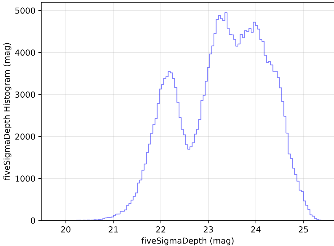
too_elab_r8_d2_ugrizy_v3.4_10yrs Yr 1 all bands: fiveSigmaDepth Histogram
