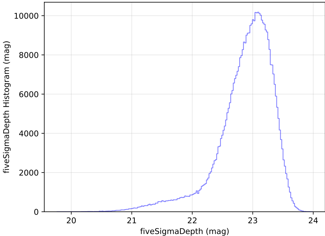
too_elab_r8_d2_ugrizy_v3.4_10yrs WFD z band: fiveSigmaDepth Histogram
