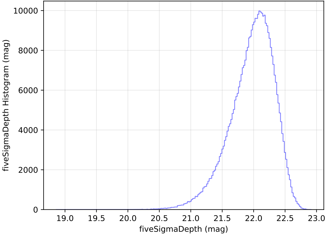
too_elab_r8_d2_ugrizy_v3.4_10yrs WFD y band: fiveSigmaDepth Histogram
