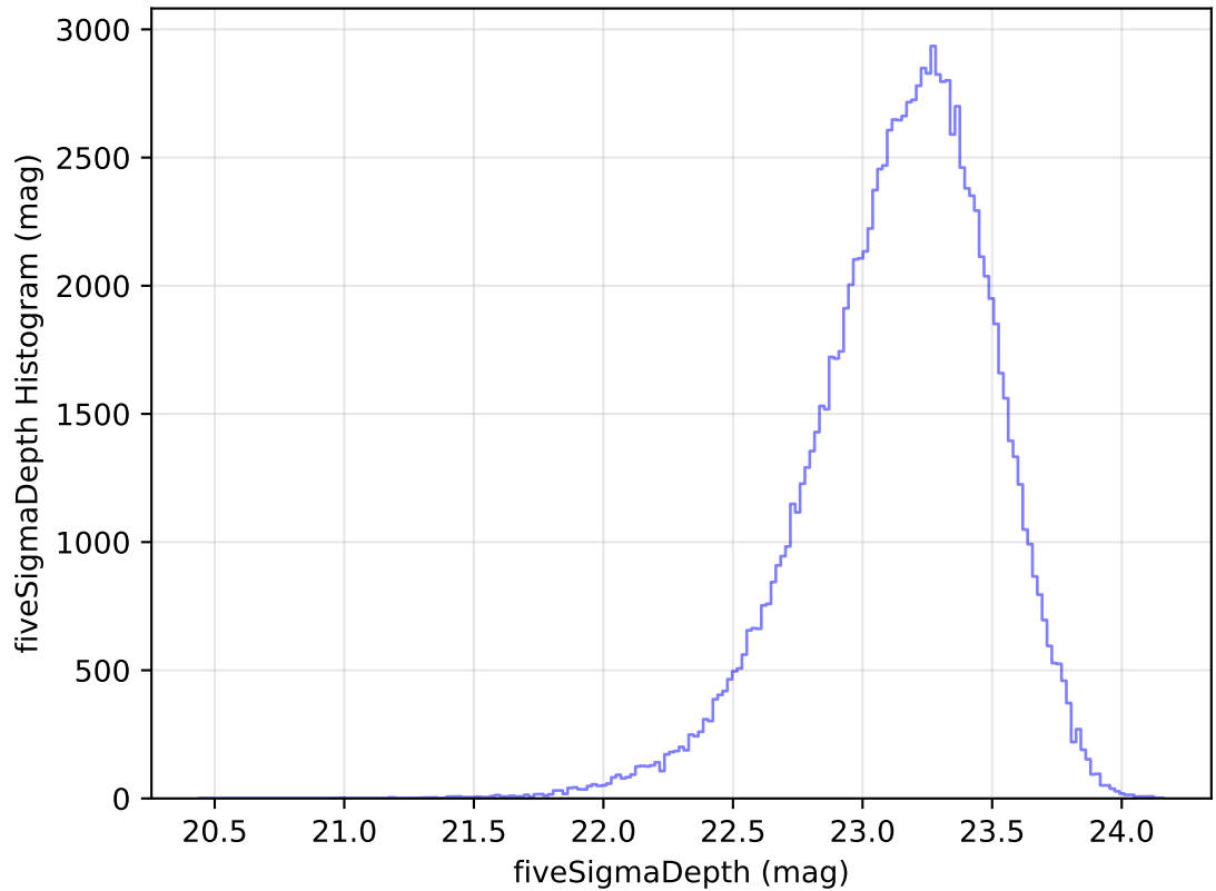
too_elab_r8_d2_ugrizy_v3.4_10yrs WFD u band: fiveSigmaDepth Histogram
