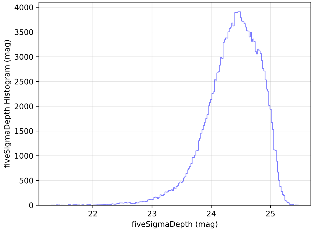
too_elab_r8_d2_ugrizy_v3.4_10yrs WFD g band: fiveSigmaDepth Histogram
