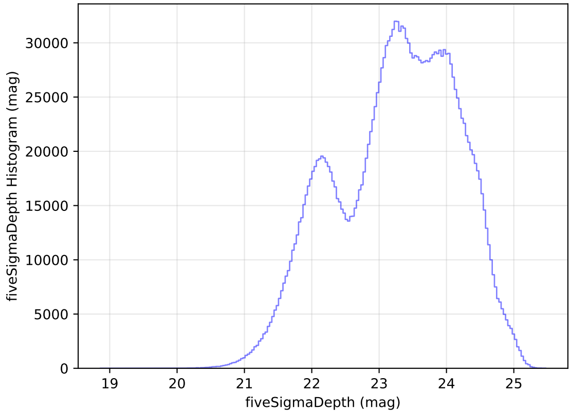
too_elab_r8_d2_ugrizy_v3.4_10yrs WFD all bands: fiveSigmaDepth Histogram
