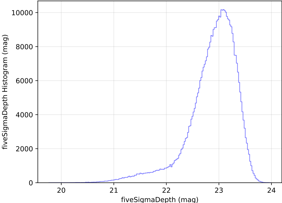
too_elab_r8_d2_ugrizy_v3.4_10yrs All sky z band: fiveSigmaDepth Histogram
