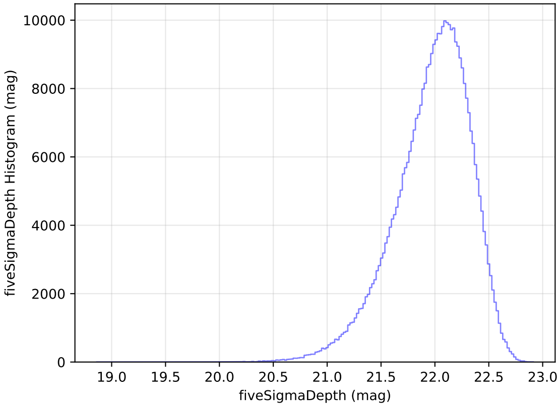
too_elab_r8_d2_ugrizy_v3.4_10yrs All sky y band: fiveSigmaDepth Histogram
