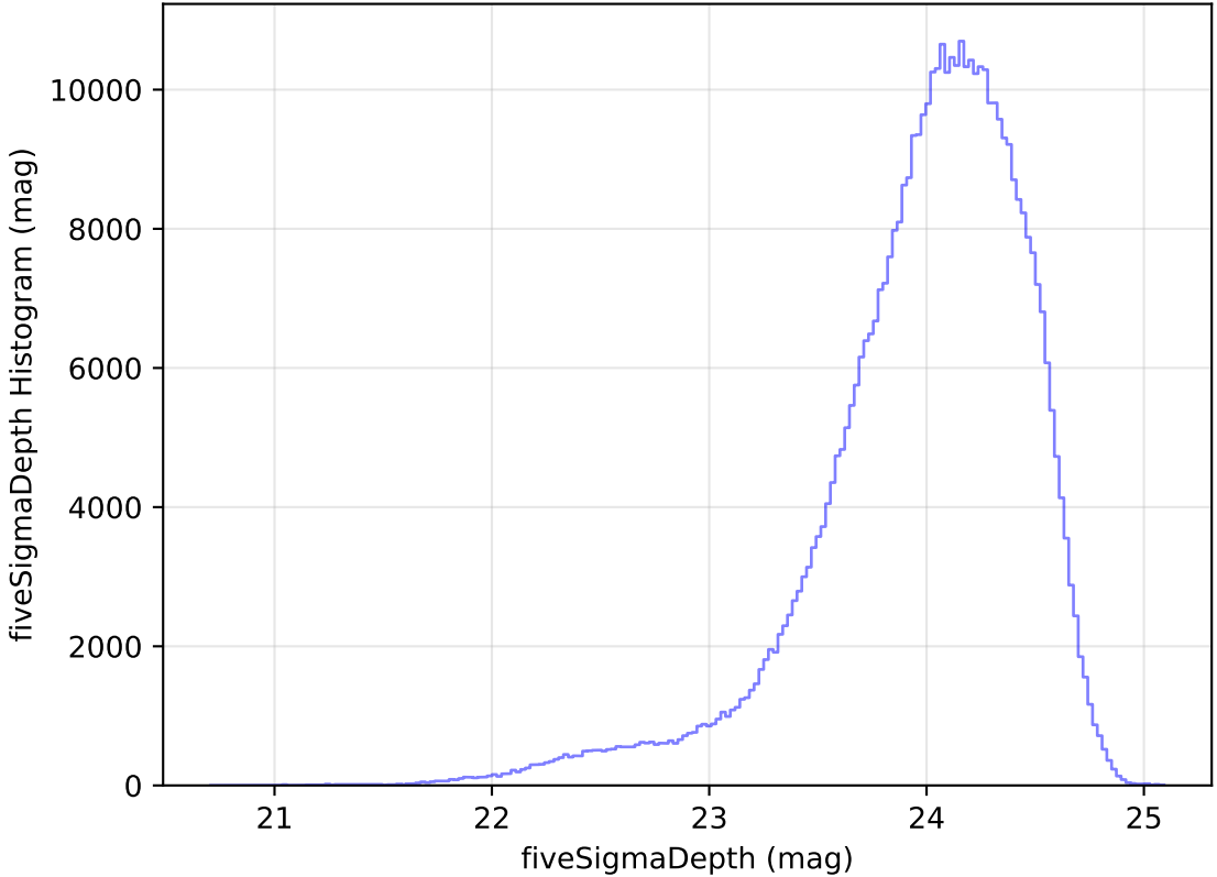
too_elab_r8_d2_ugrizy_v3.4_10yrs All sky r band: fiveSigmaDepth Histogram
