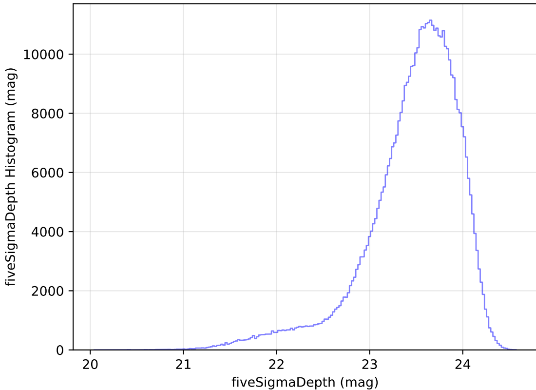
too_elab_r8_d2_ugrizy_v3.4_10yrs All sky i band: fiveSigmaDepth Histogram
