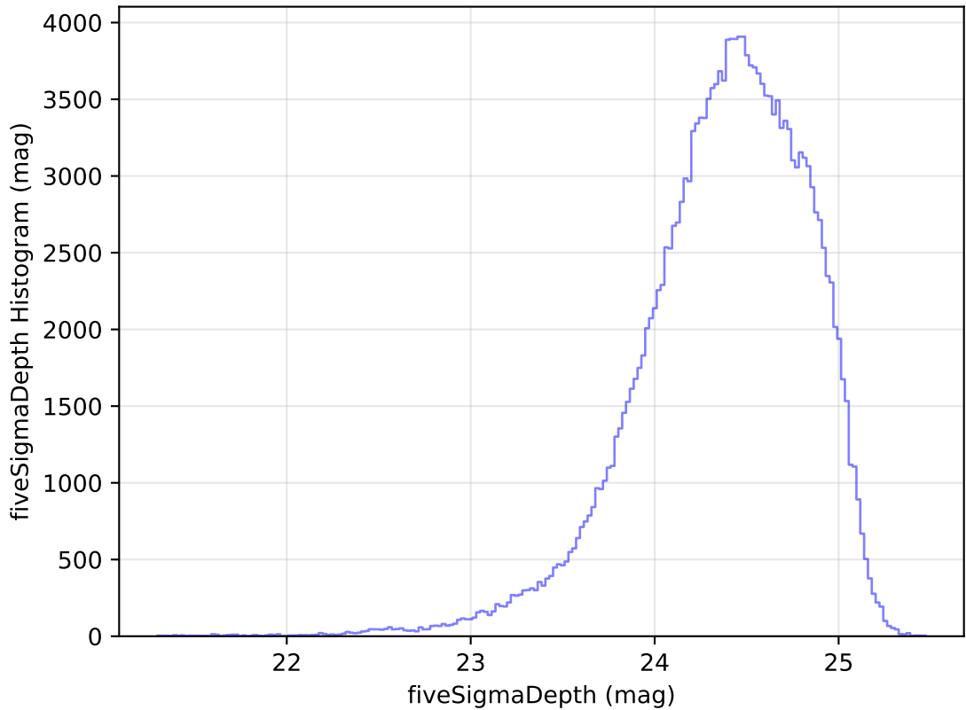
too_elab_r8_d2_ugrizy_v3.4_10yrs All sky g band: fiveSigmaDepth Histogram
