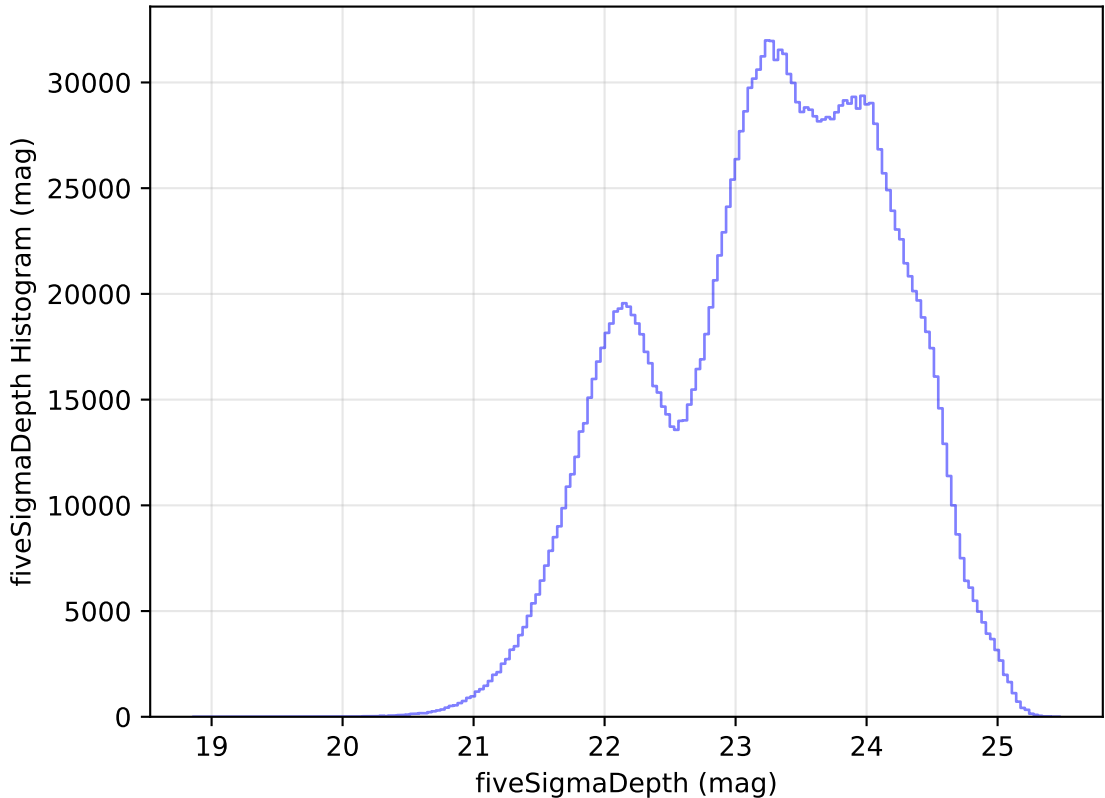
too_elab_r8_d2_ugrizy_v3.4_10yrs All sky all bands: fiveSigmaDepth Histogram
