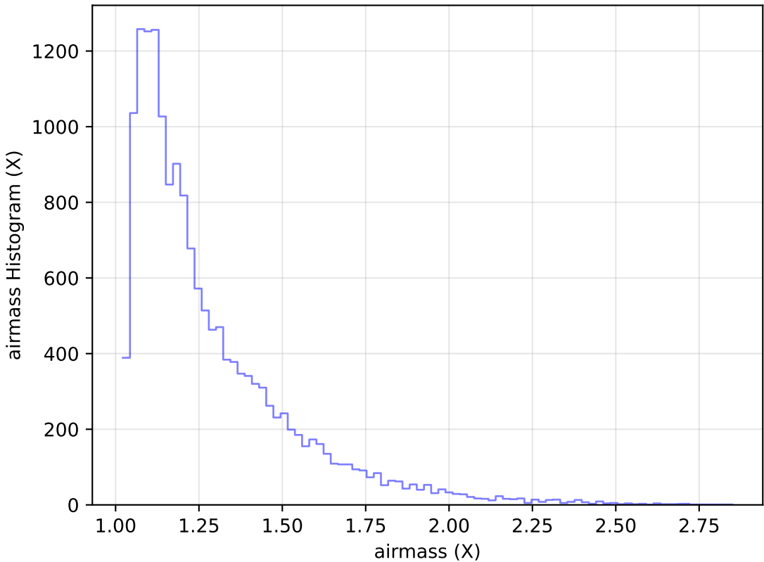
too_elab_r8_d2_ugrizy_v3.4_10yrs Yr 1 u band: airmass Histogram
