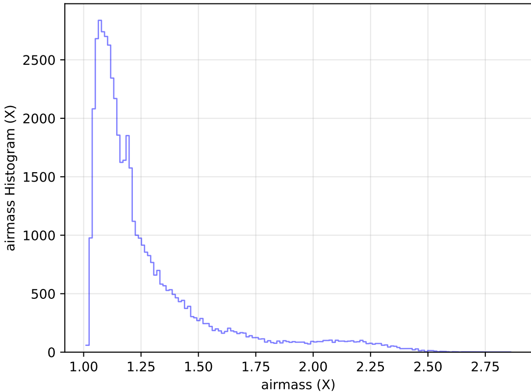
too_elab_r8_d2_ugrizy_v3.4_10yrs Yr 1 r band: airmass Histogram
