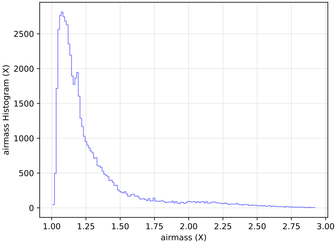
too_elab_r8_d2_ugrizy_v3.4_10yrs Yr 1 i band: airmass Histogram
