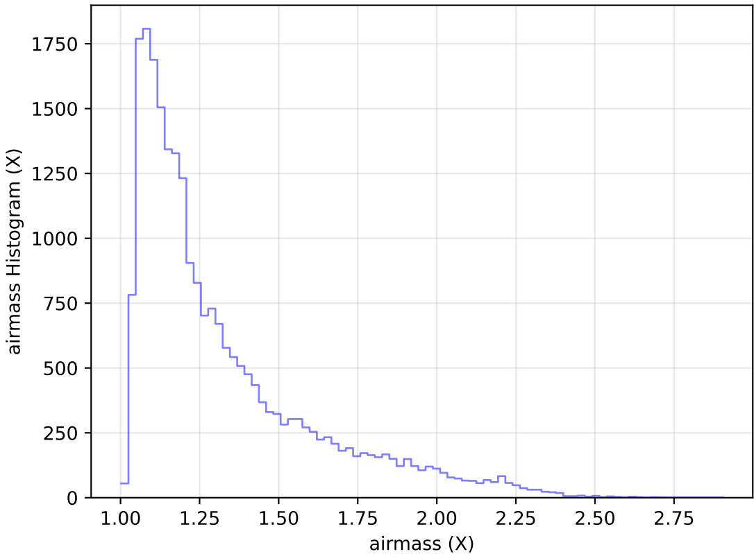
too_elab_r8_d2_ugrizy_v3.4_10yrs Yr 1 g band: airmass Histogram
