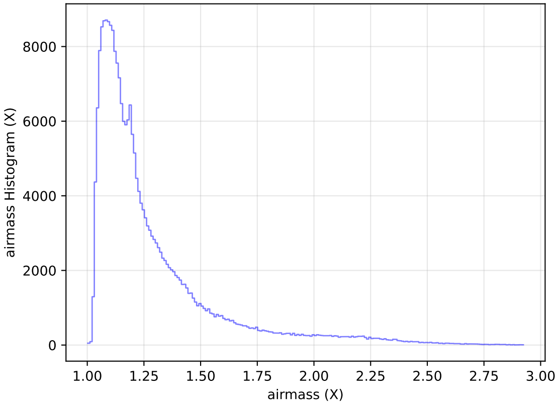
too_elab_r8_d2_ugrizy_v3.4_10yrs Yr 1 all bands: airmass Histogram
