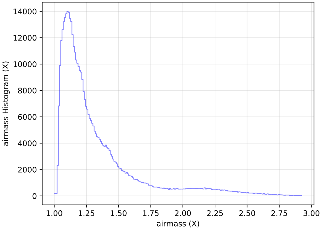
too_elab_r8_d2_ugrizy_v3.4_10yrs WFD z band: airmass Histogram
