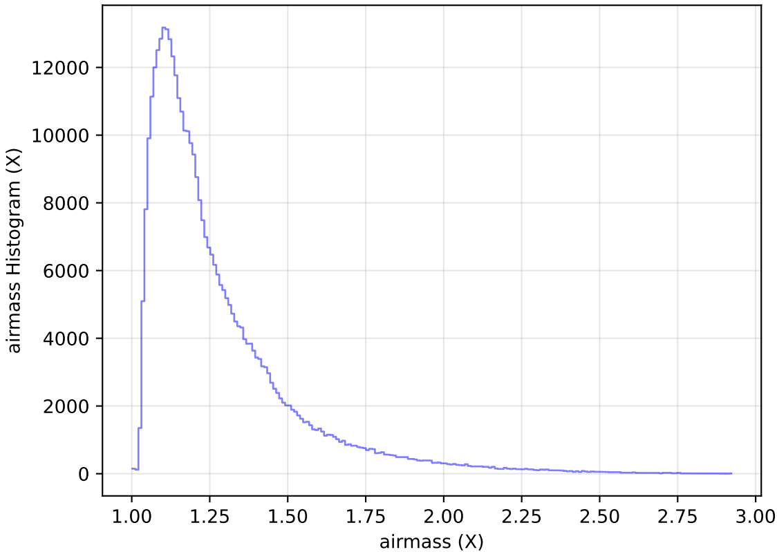
too_elab_r8_d2_ugrizy_v3.4_10yrs WFD y band: airmass Histogram
