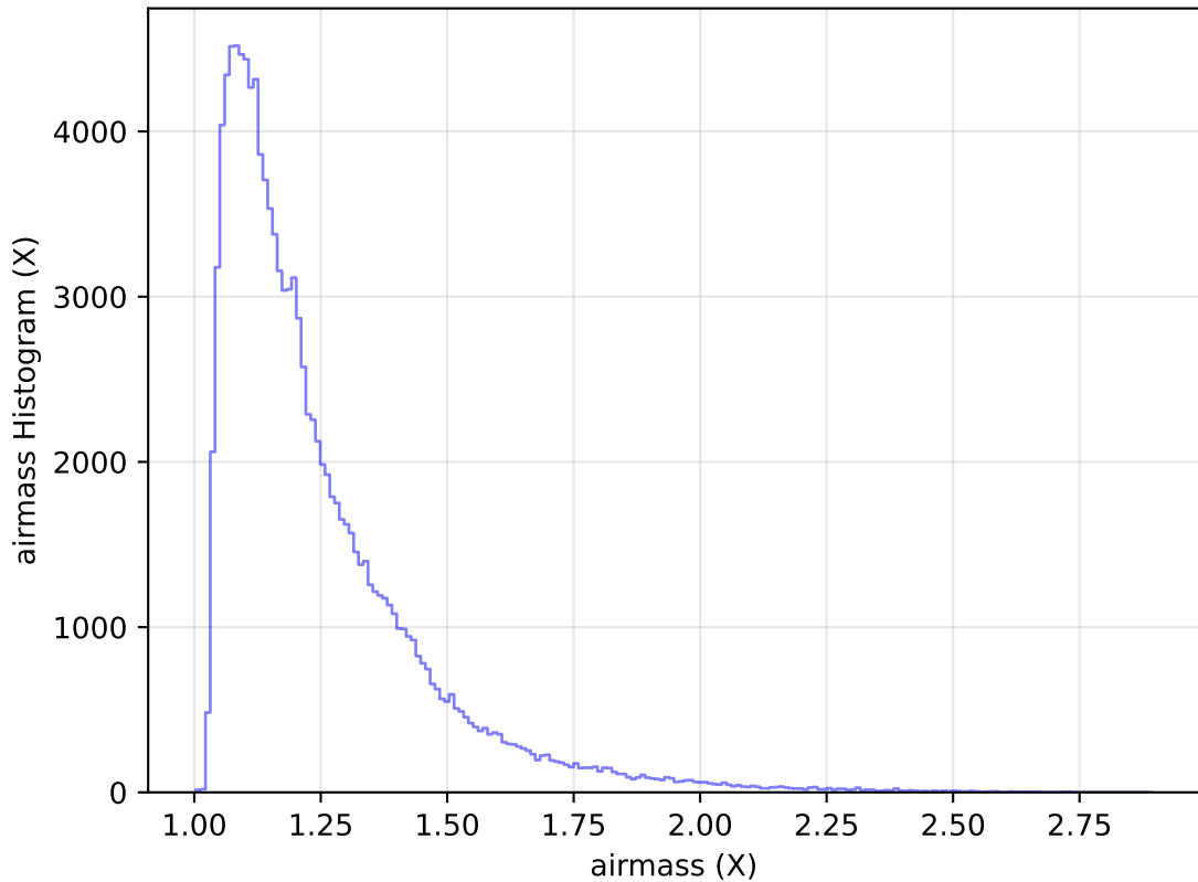
too_elab_r8_d2_ugrizy_v3.4_10yrs WFD u band: airmass Histogram
