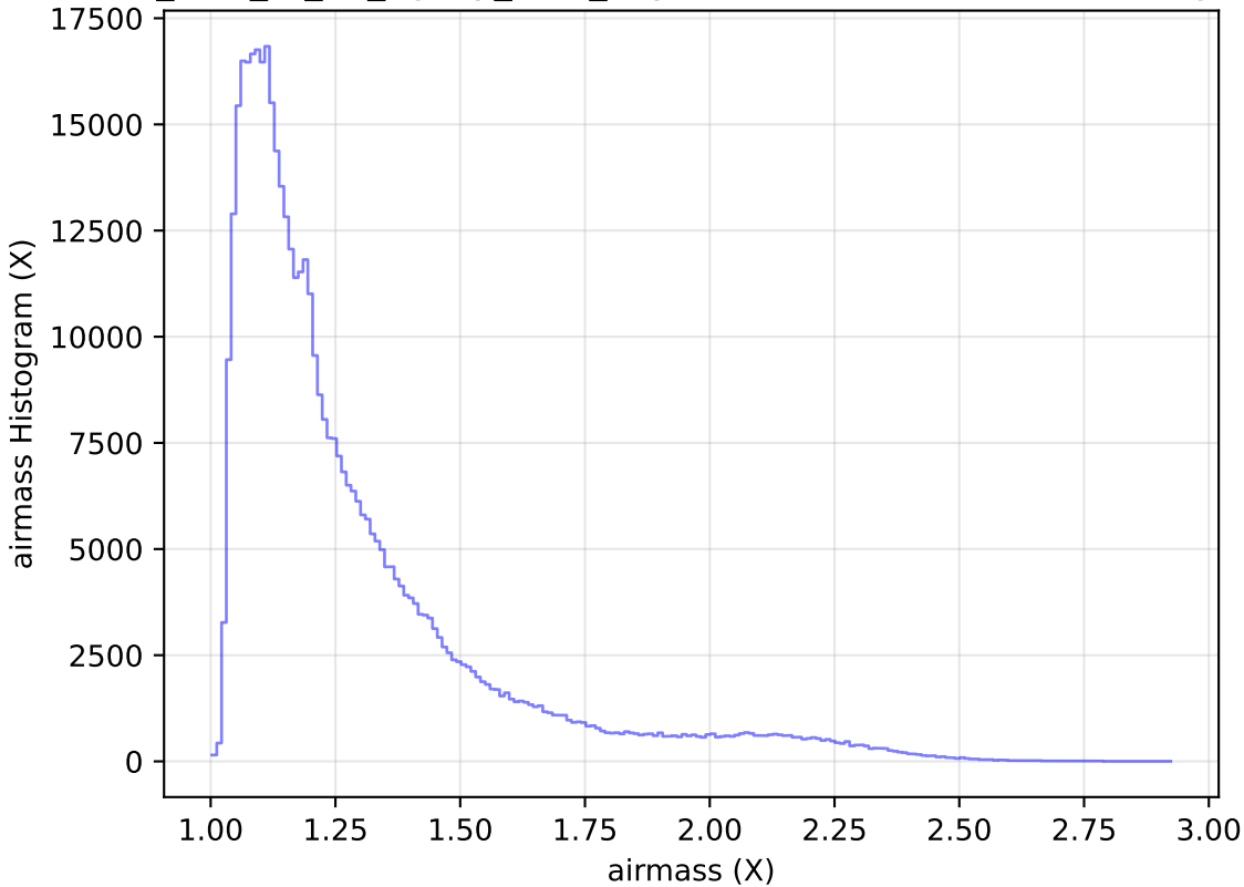
too_elab_r8_d2_ugrizy_v3.4_10yrs WFD r band: airmass Histogram
