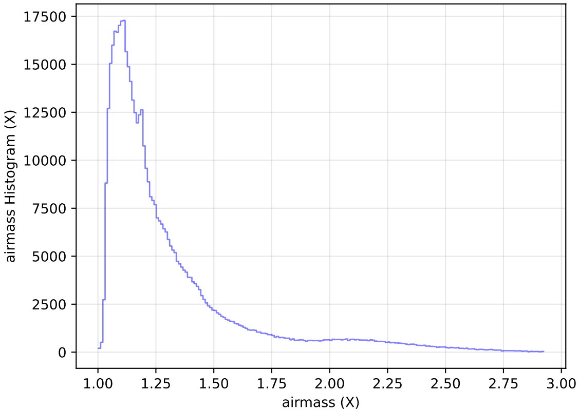
too_elab_r8_d2_ugrizy_v3.4_10yrs WFD i band: airmass Histogram
