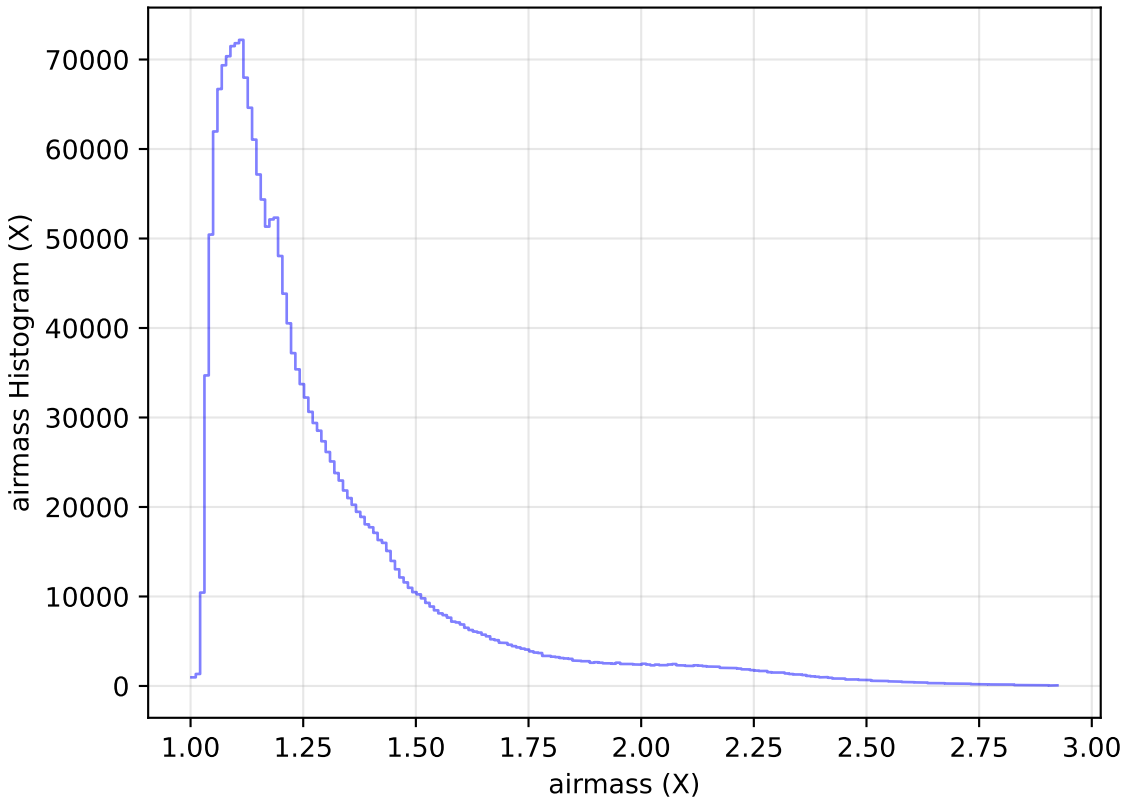
too_elab_r8_d2_ugrizy_v3.4_10yrs WFD all bands: airmass Histogram
