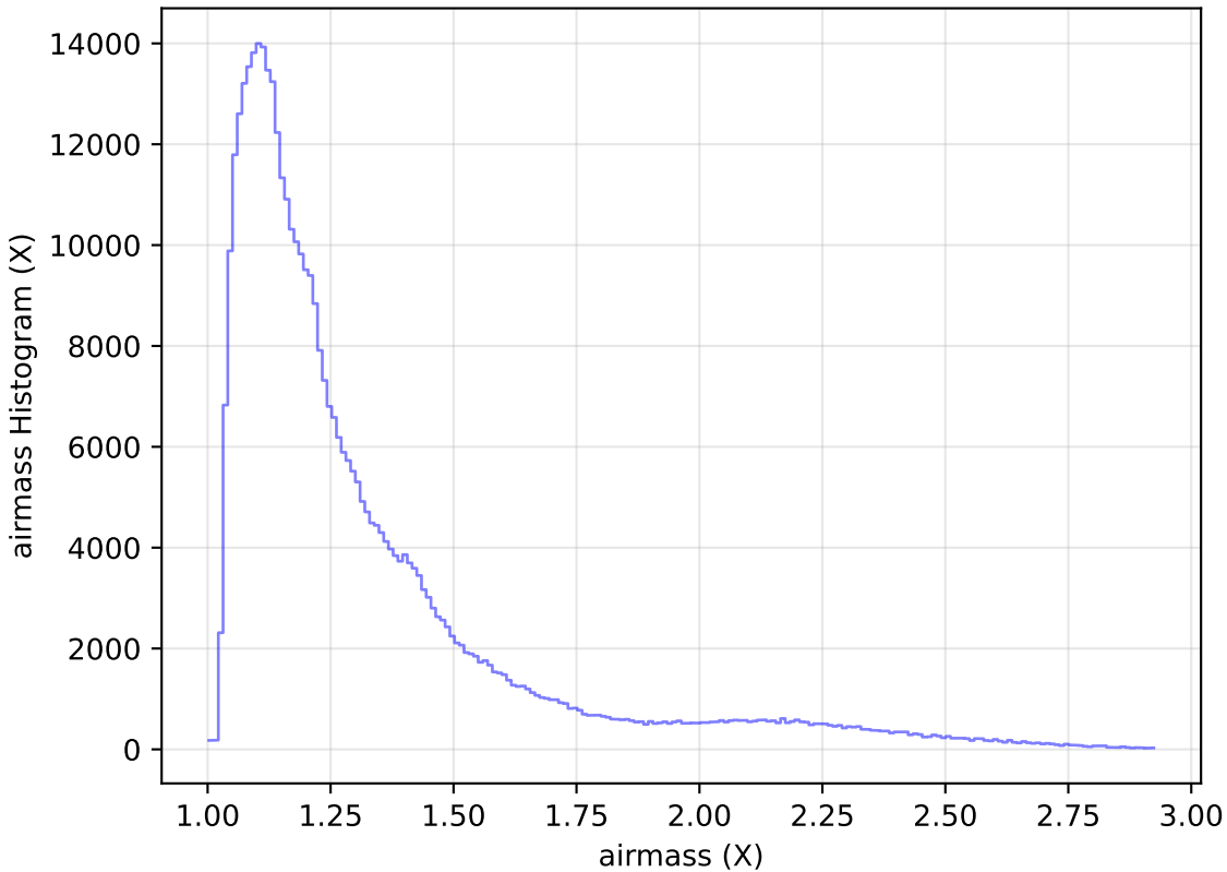
too_elab_r8_d2_ugrizy_v3.4_10yrs All sky z band: airmass Histogram
