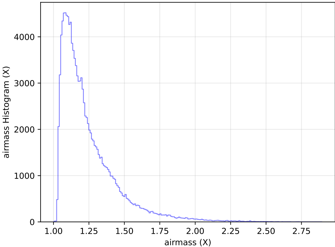
too_elab_r8_d2_ugrizy_v3.4_10yrs All sky u band: airmass Histogram
