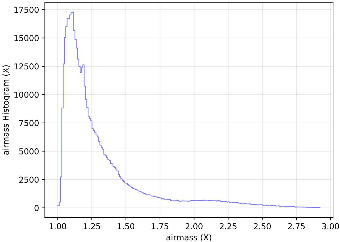
too_elab_r8_d2_ugrizy_v3.4_10yrs All sky i band: airmass Histogram
